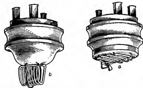
FIG. 18.—Nernst Lamp, Burners for B Type. a, low voltage; b, high voltage.
