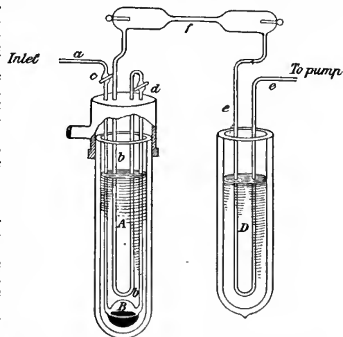
FIG. 9.—Apparatus for continuous Spectroscopic Examination.
