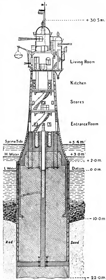
FIG. 21.—Rothersand Lighthouse.
