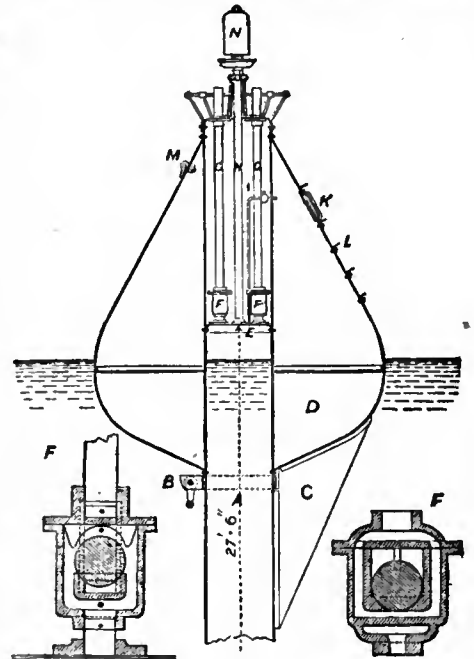
FIG. 51.—Courtenay's Automatic Whistling Buoy.
