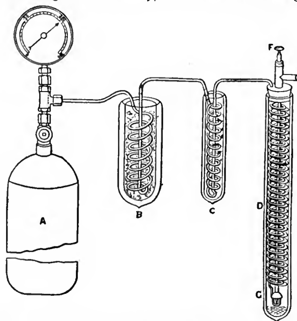
FIG. 3.—Hydrogen Jet Apparatus. A, Cylinder containing compressed hydrogen. B and C, Vacuum vessels containing carbonic acid under exhaustion and liquid air respectively. D, Regenerating coil in vacuum vessel. F, Valve. G, Pin-hole nozzle.
