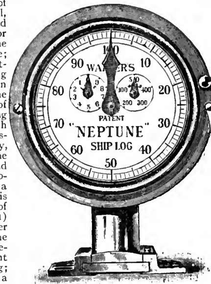
FIG. 7.—Dial-plate of Neptune Log.
