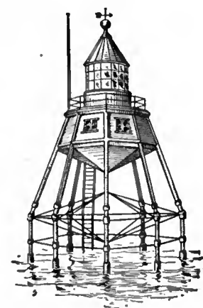
FIG. 19.—Maplin Pile Lighthouse.
