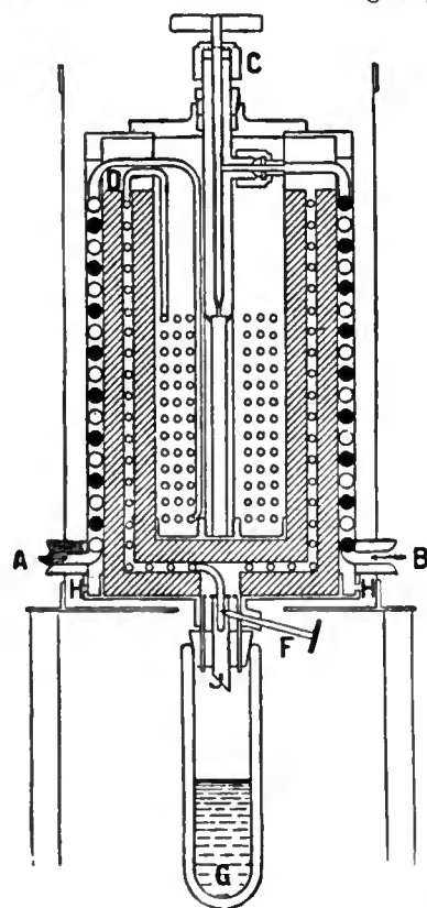
FIG. 2.—Laboratory Liquid Air Machine.
