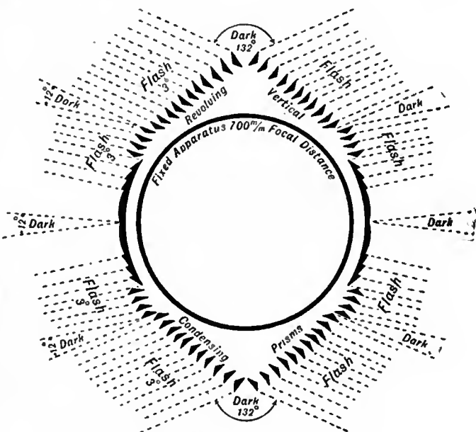
FIG. 45.—Isle of May Apparatus.
