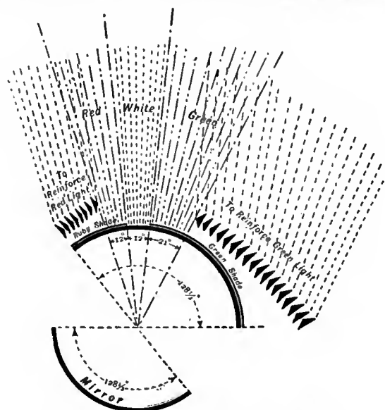
FIG. 38.—Gage Roads Direction Light.
