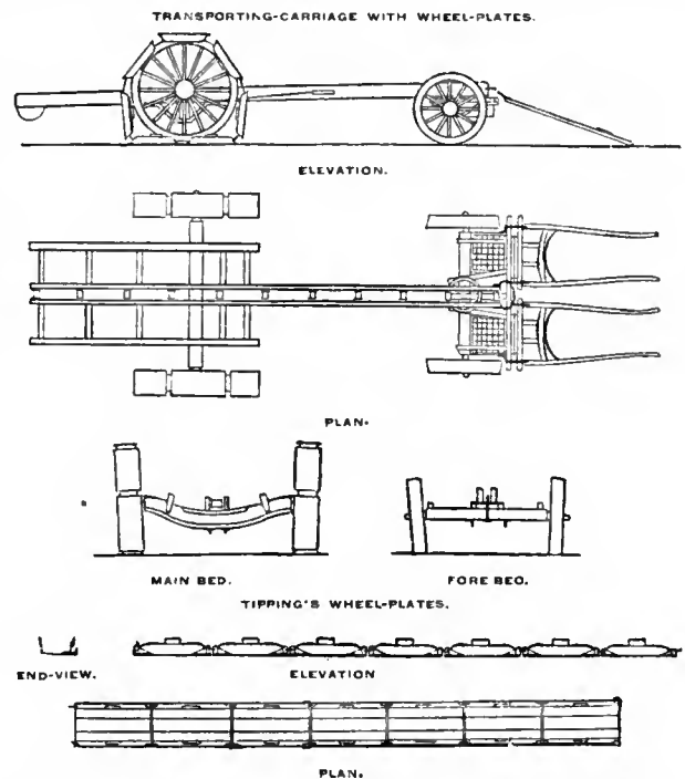
FIG. 9.—Life-boat Transporting-Carriage with Tipping's Wheel-Plates.
