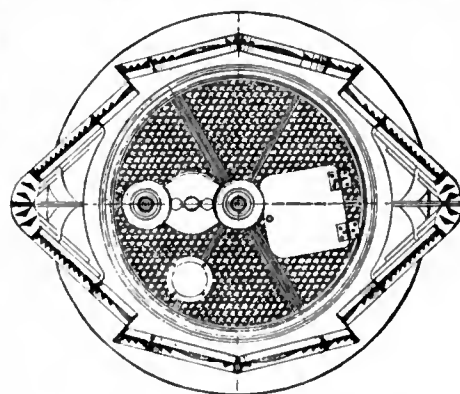
FIG. 39.—Pendeen Apparatus. Plan at Focal Plane.
