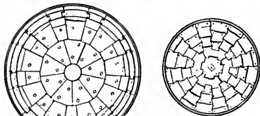
Eddystone, 12th Course, Smeaton's Tower.
