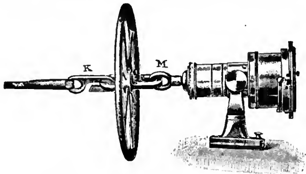
FIG. 11.—Neptune Log fitted with Governor.
