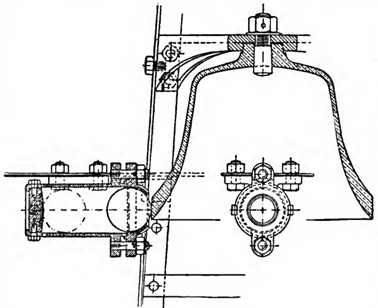
FIG. 52.—Buoy Bell.
