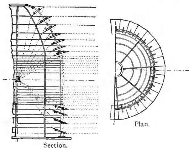
FIG. 35.—Fixed Apparatus at Chassiron Lighthouse (1827).
