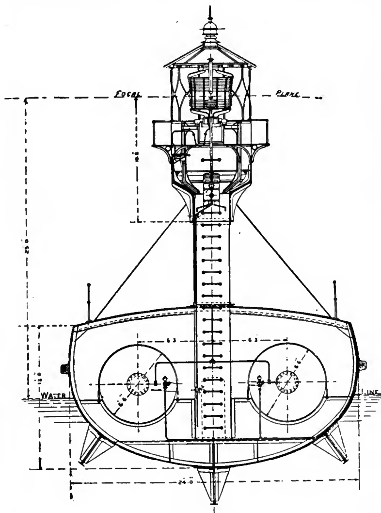
FIG. 49.—Otter Rock Light-vessel.
