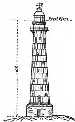
FIG. 25.—Dassen Island Lighthouse (cast iron).
