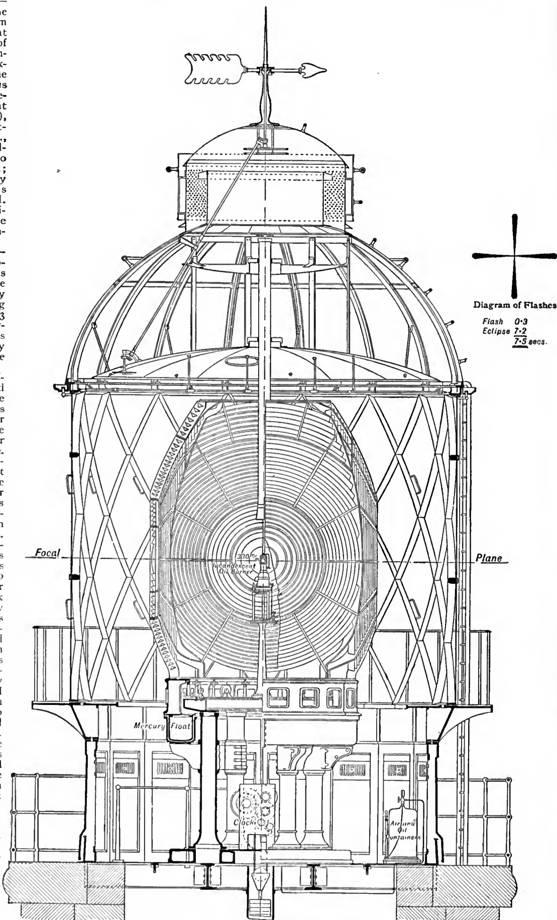
FIG. 41.—Manora Point Apparatus and Lantern.
