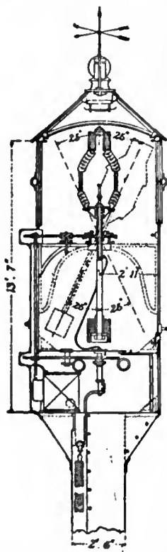
FIG. 48.—Lantern of Sandettié Lightship.
