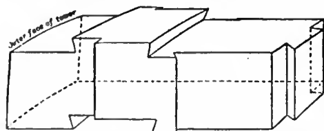
FIG. 23.—Perspective drawing of Dovetailed Stone (Wolf Rock).
