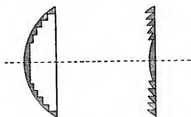
FIG. 32. Fresnel's Annular Lens.
