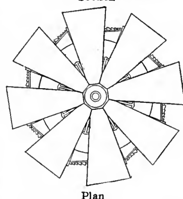
FIG. 34.—Fresnel's Revolving Apparatus at Cordouan Lighthouse.
