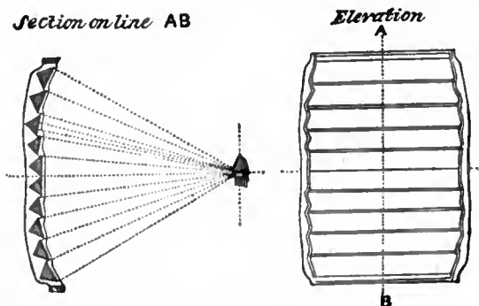
FIG. 37.—Chance's Dioptric Spherical Mirror.
