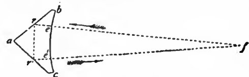
FIG. 36.—Vertical Section. Prism of Dioptric Spherical Mirror.
