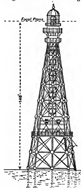
FIG. 26.—Cape San Thomé Lighthouse.
