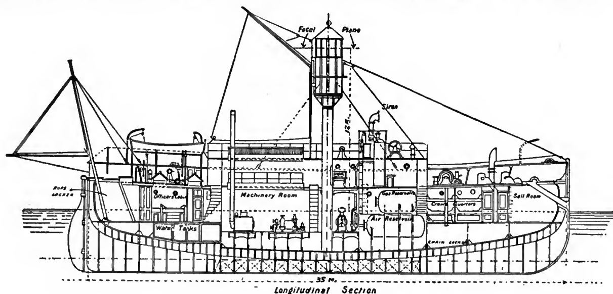
FIG. 47.—Sandettié Lightship.
