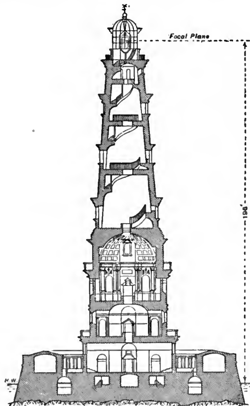
FIG. 1.—Cordouan Lighthouse.
