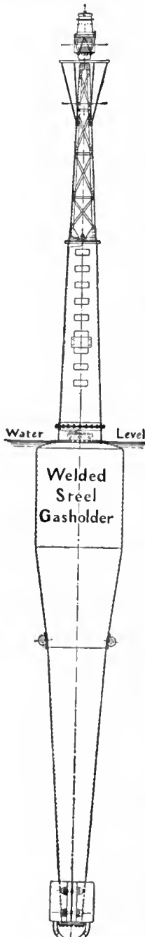
FIG. 50.—Spar Gas Buoy.
