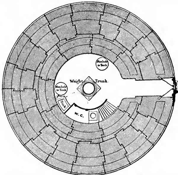
FIG. 6.—Plan of Entrance Floor, Eddystone Lighthouse.
